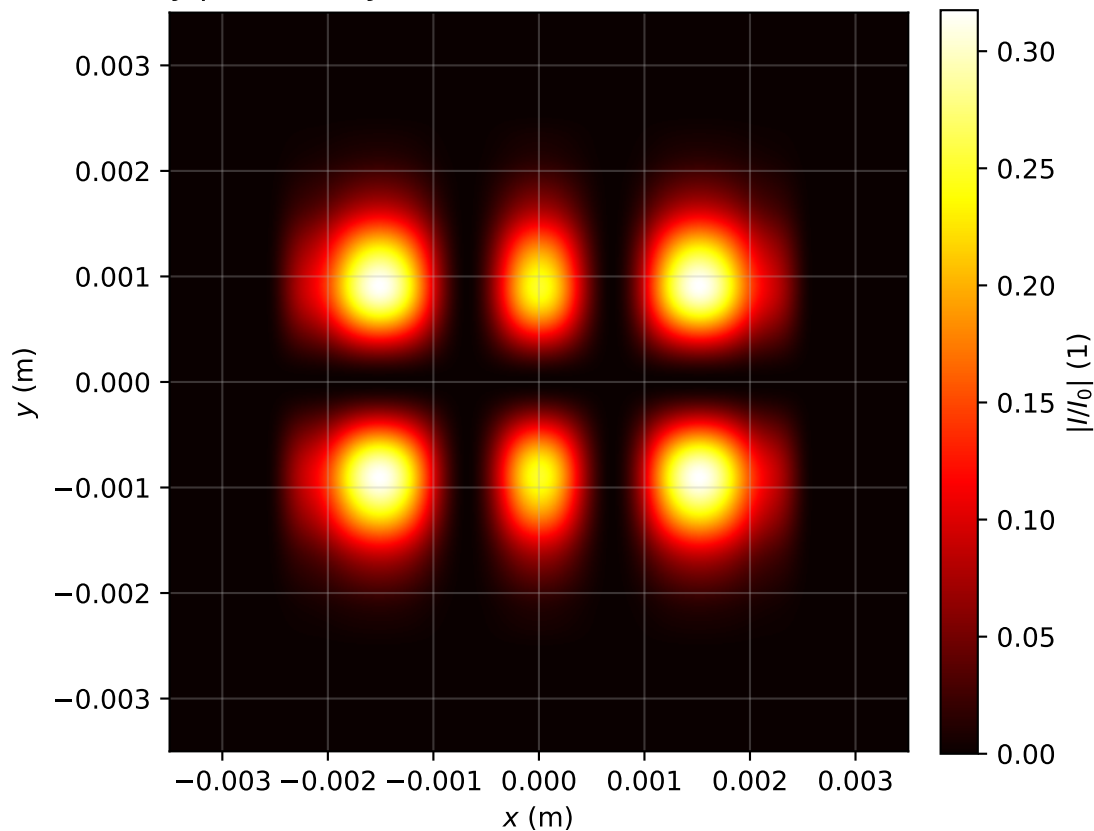
Intensity profile I(x, y, z = 3.264)/I_0 , P_{in}=1.0P_{cr} , artificial time
